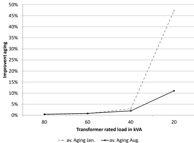
Fig. 3. Improvement average aging, 10 households.
