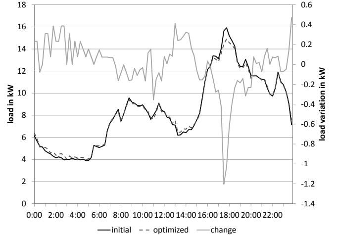
Fig. 1. Average daily load curve January, 10 households, max. 3.5 kWh shifted Energy.
