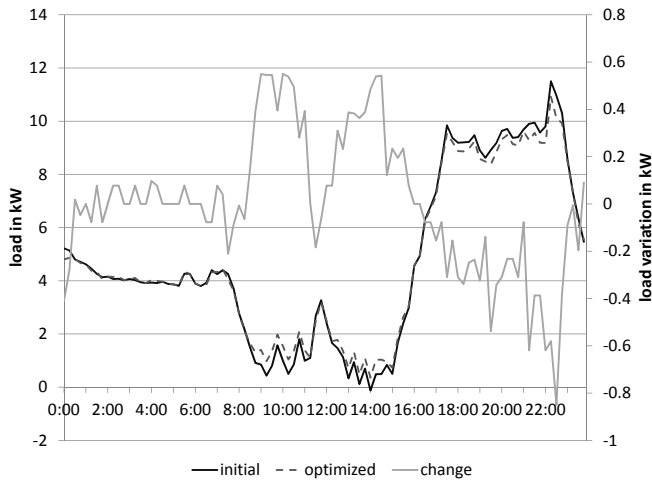
Fig. 2. Average daily load curve August, 10 households, max. 3.5 kWh shifted Energy.
