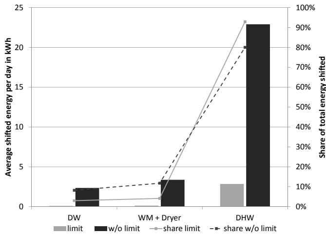
Fig. 6. Share of devices on shifted load without limit.
