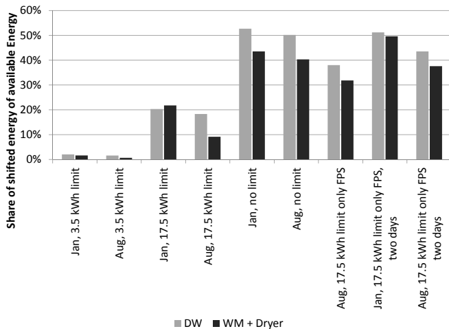
Fig. 7. Share shifted energy of total energy for FPS devices.
