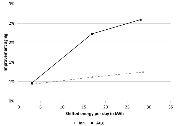
Fig. 4. Relation between shifted energy and improvement Aging, 80 kVA
