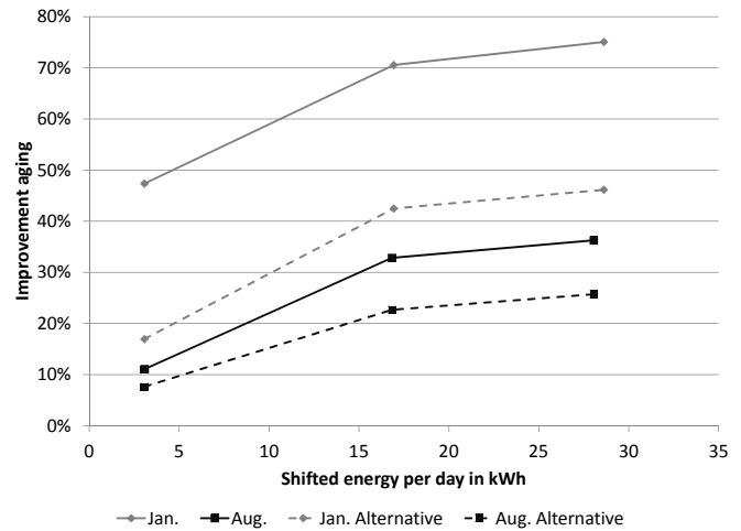
Fig. 5. Relation between shifted energy and improvement Aging, 20 kVA.
