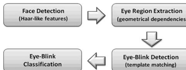
Fig. 3 Scheme of the proposed algorithm for eye-blink detection
